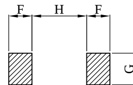
( PCB Pattern )
